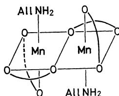
Fig. 5. A proposed structure of dimeric bis(acetylacetonato)-allylaminemanganese(II).
